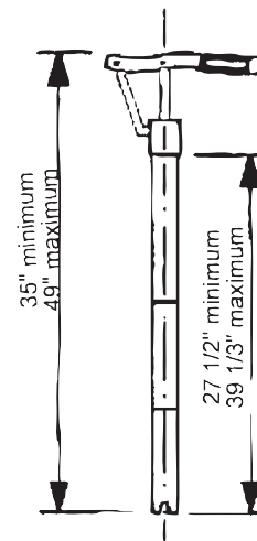
16-gallon Drum
