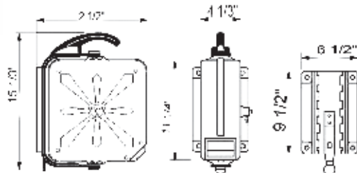
Wall-mounted
